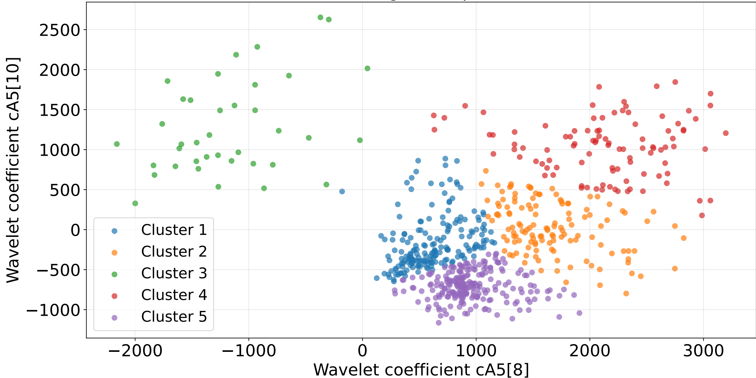
K-means clustering result (predicted labels)
